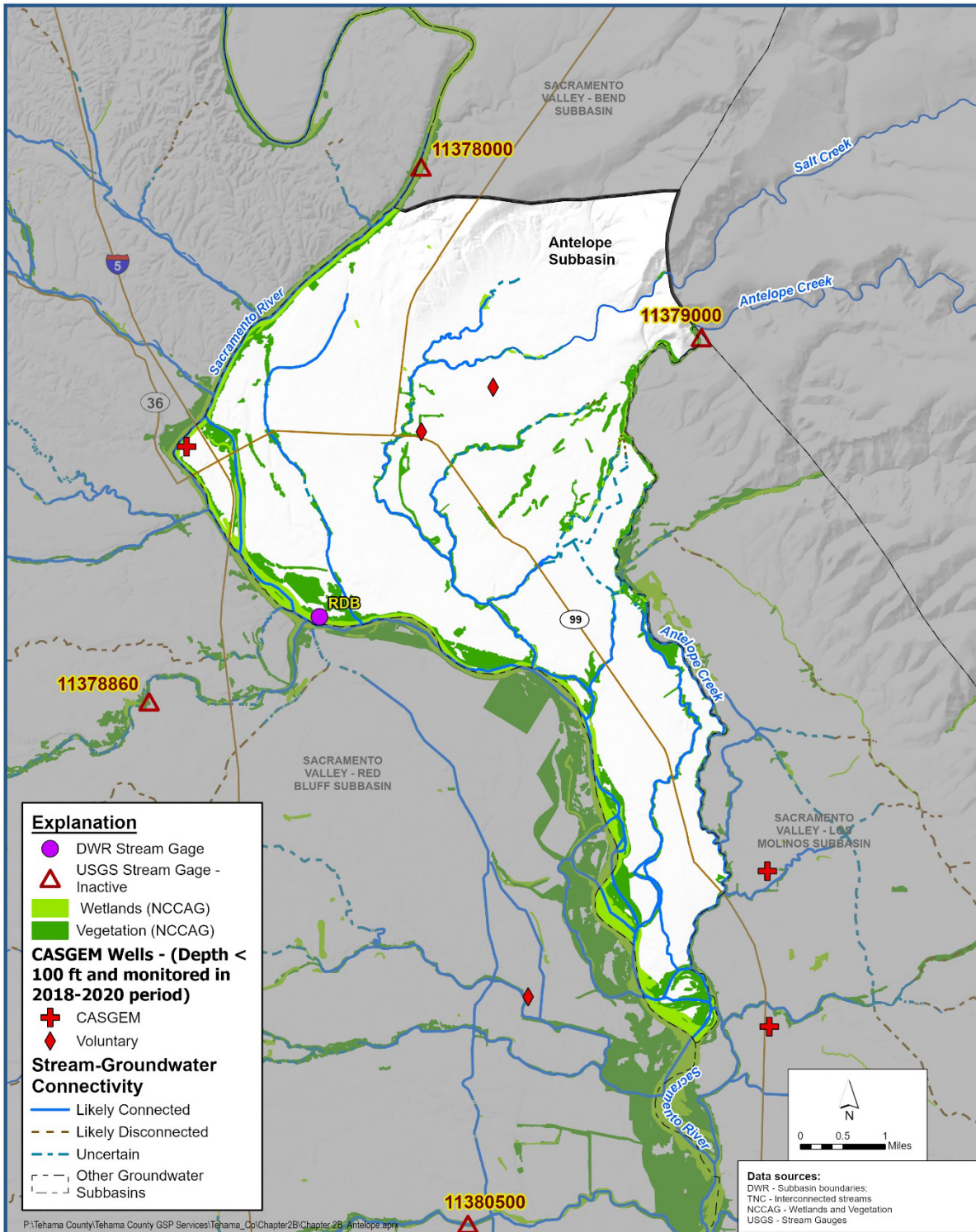
Surface Water and Shallow Groundwater Monitoring Stations Groundwater Sustainability Plan Antelope Subbasin
