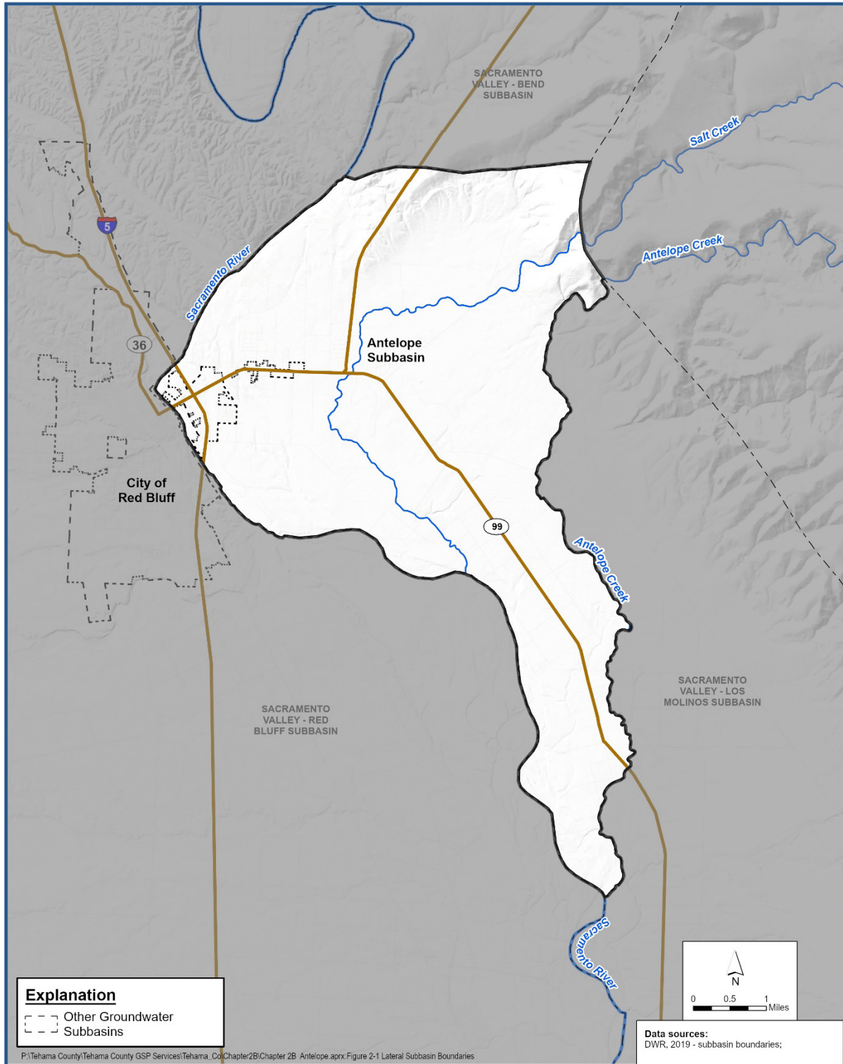
Lateral Subbasin Boundary Groundwater Sustainability Plan Antelope Subbasin
