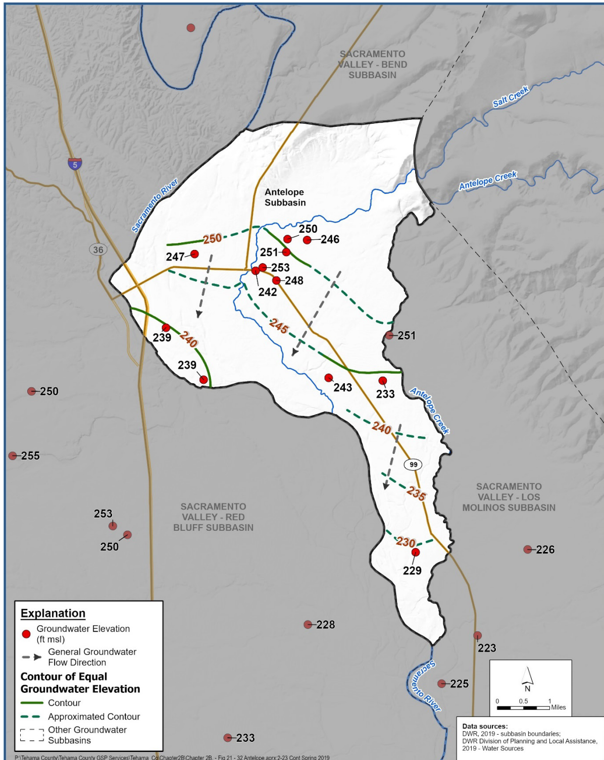
Contours of Equal Groundwater Elevation Upper Aquifer - Seasonal High of 2019 Groundwater Sustainability Plan Antelope Subbasin
