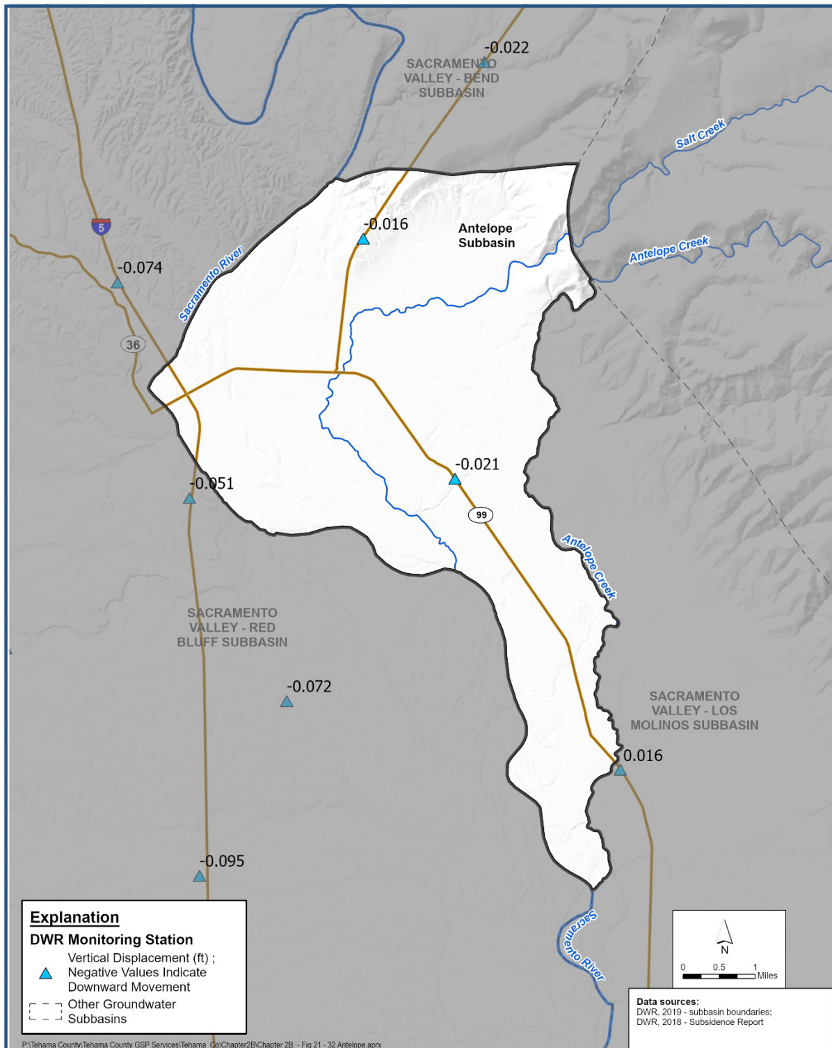
Subsidence Measurements Between 2008 and 2017 Groundwater Sustainability Plan Antelope Subbasin
