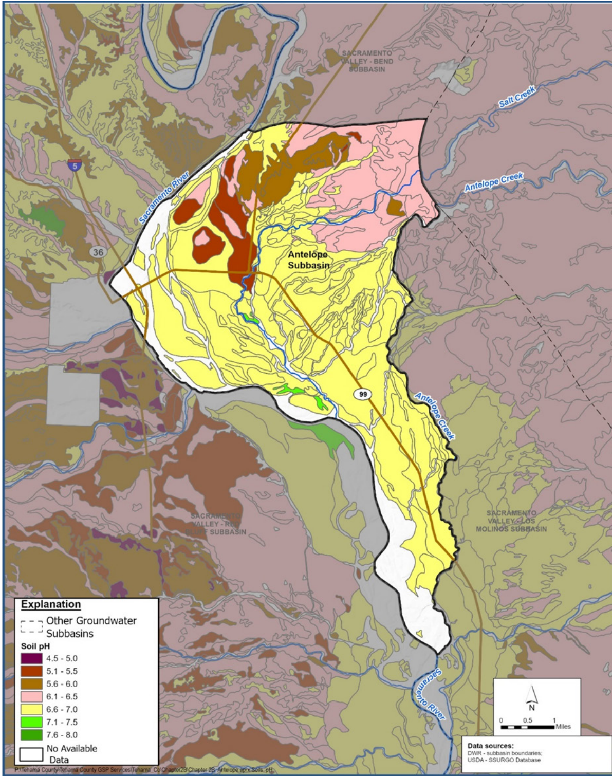
Soils - pH Groundwater Sustainability Plan Antelope Subbasin
