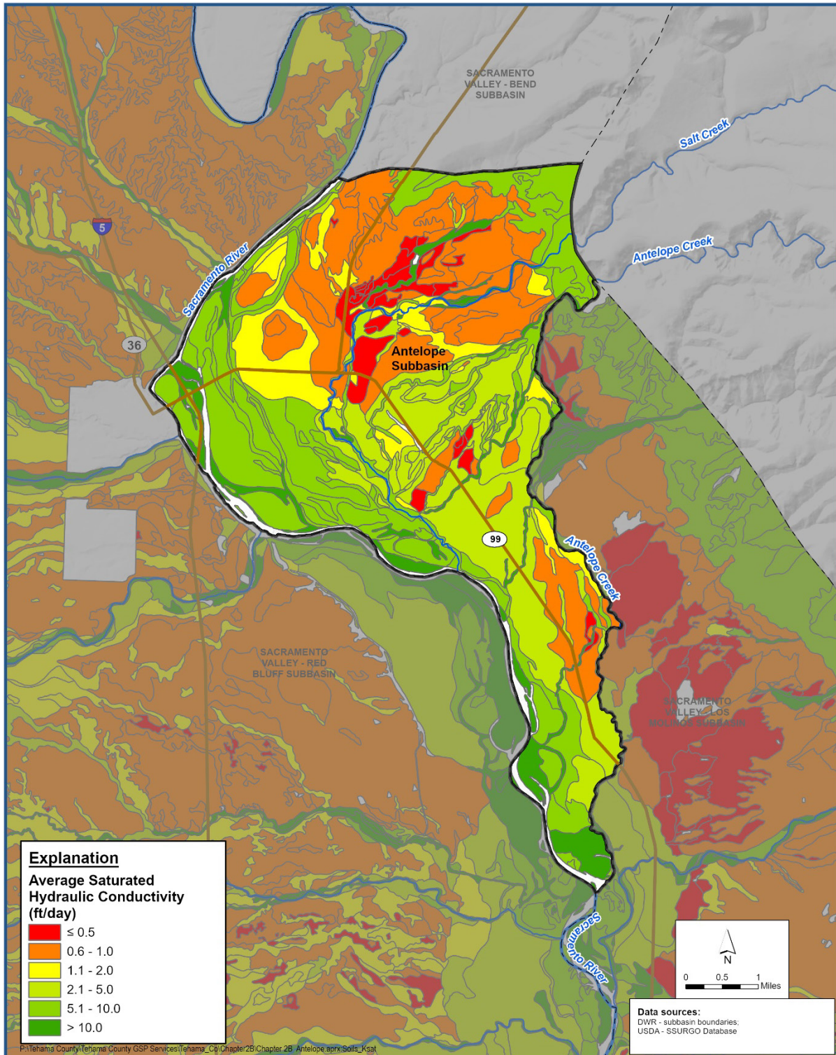
Soils - Saturated Hydraulic Conductivity Groundwater Sustainability Plan Antelope Subbasin
