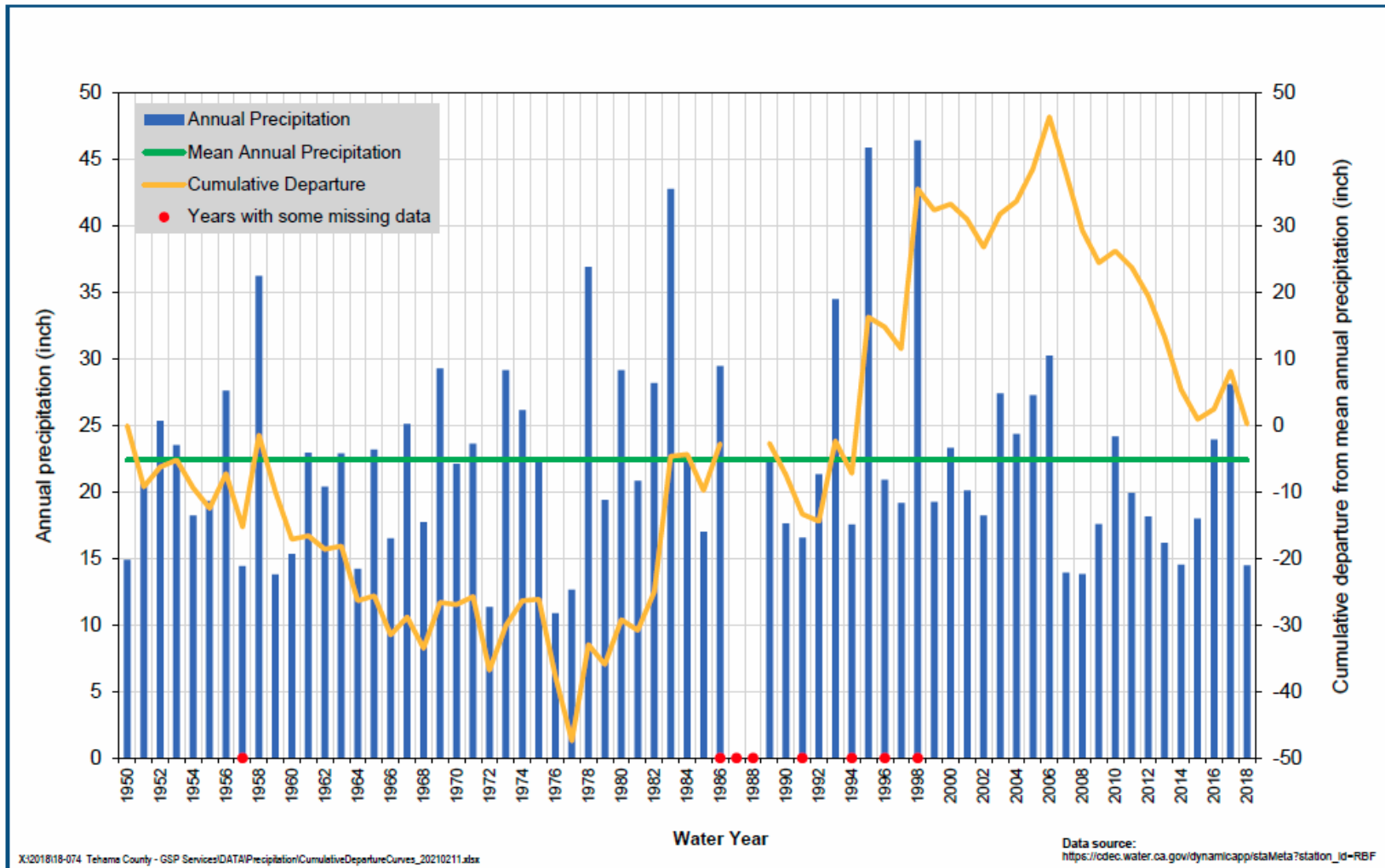
Annual Precipitation and Cumulative Departure at Red Bluff Municipal Airport Groundwater Sustainability Plan Antelope Subbasin
