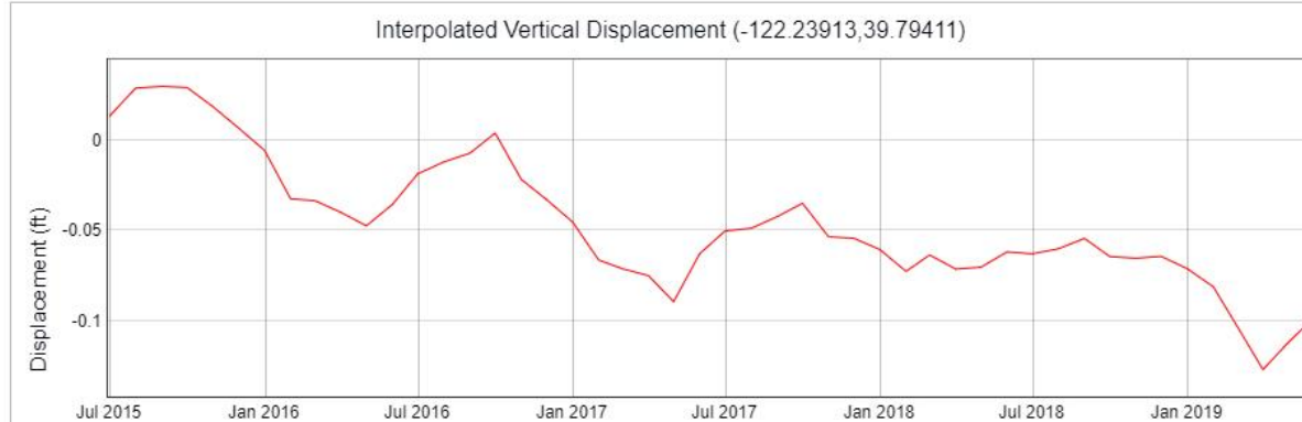
Figure 3-35. DWR InSAR Subsidence from June 2015 to June 2019 Near Sacramento Valley Subsidence Survey Location 2966. 27
