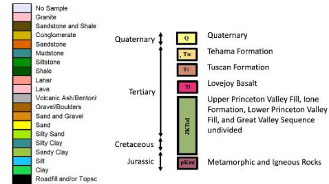
Figure 3-13. East-West AEM Cross Section in Eastern Corning Subbasin near Hamilton City
