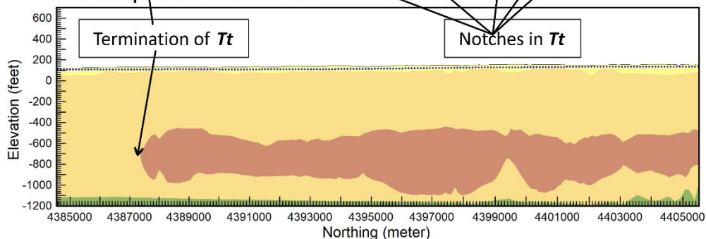
Figure 3-14. North-South AEM Cross Section in Eastern Corning Subbasin near Hamilton City
