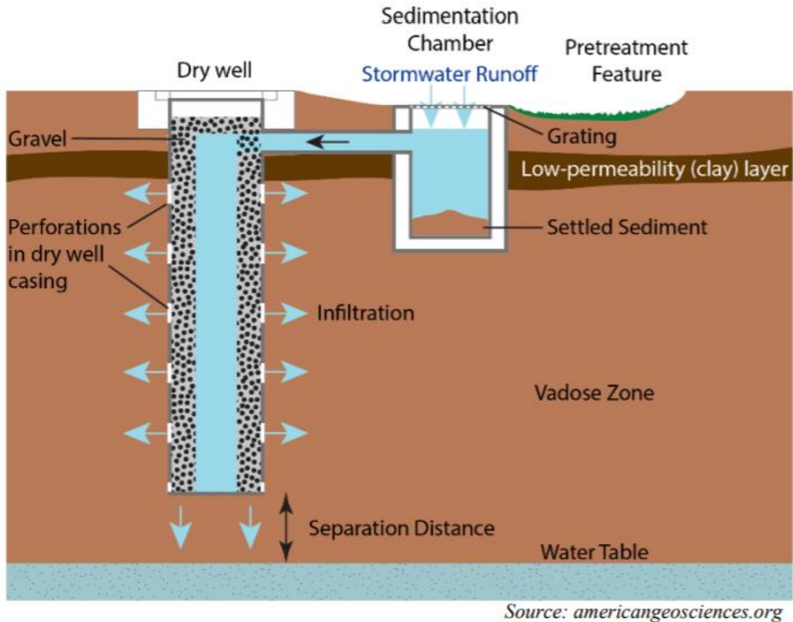
Figure 7-16. Typical Schematic for Dry Well Stormwater Recharge System (SWRCB, 2020)
