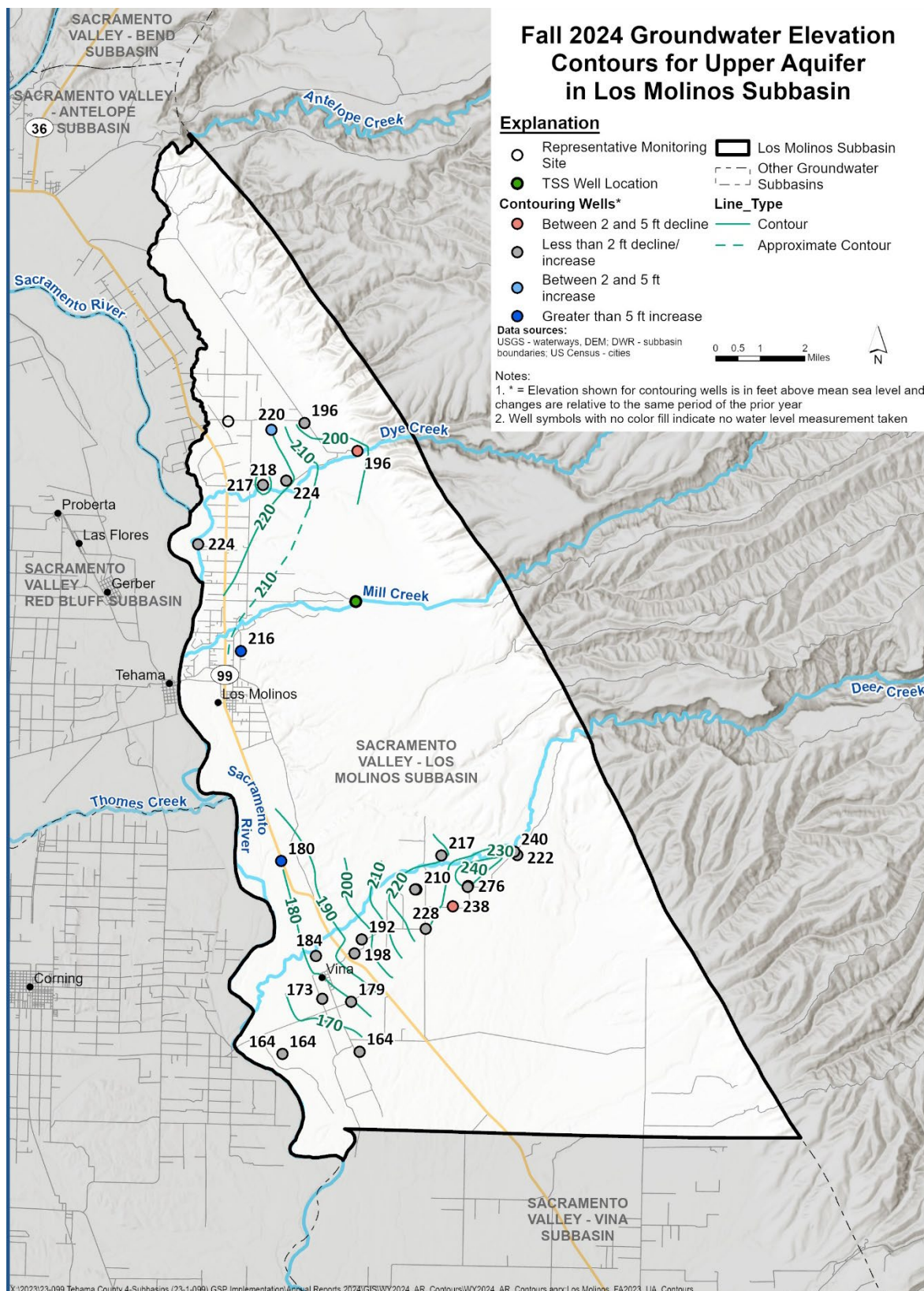
Figure 2-2. Los Molinos Subbasin Contours of Equal Groundwater Elevation for the Upper Aquifer, Fall 2024 (Seasonal Low)
