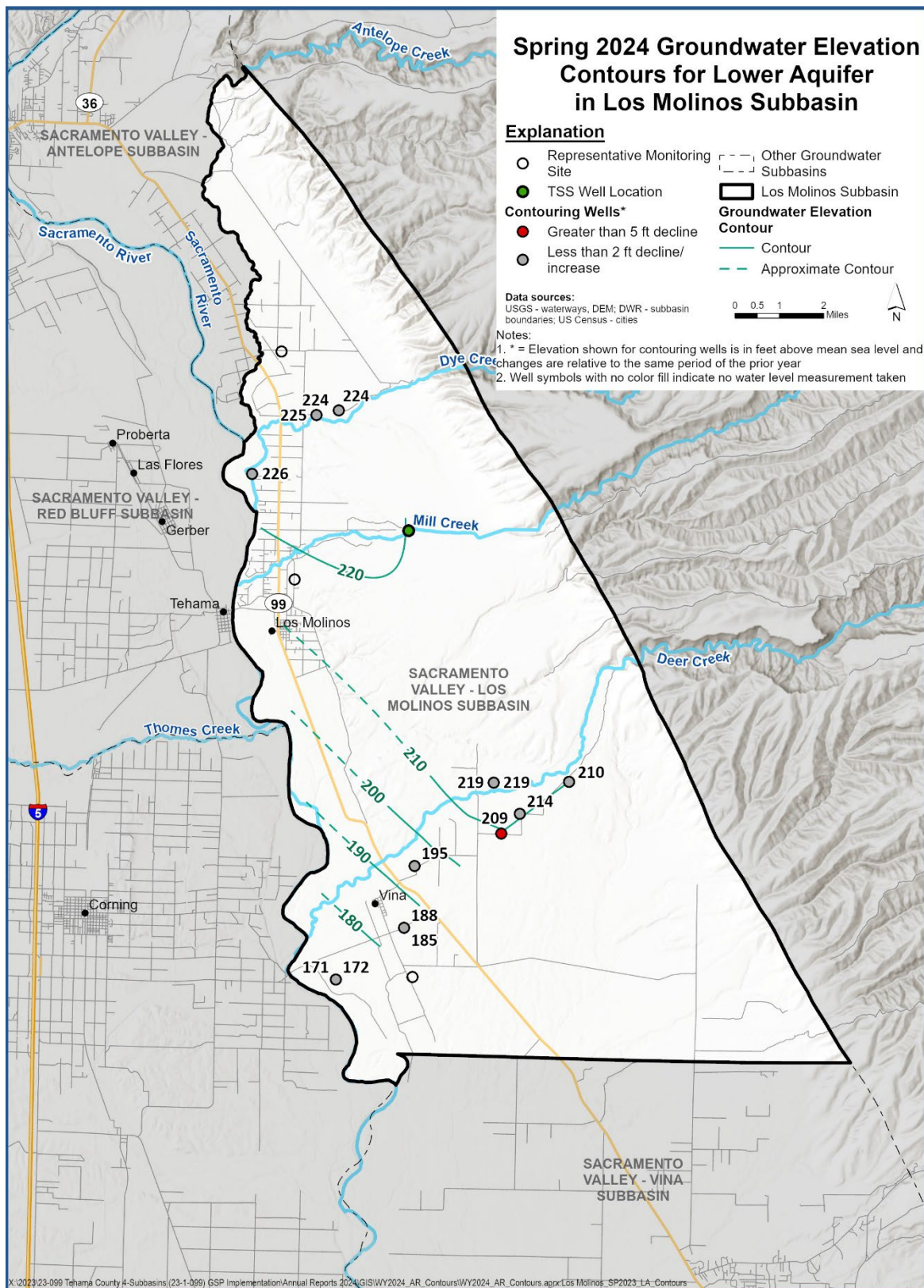
Figure 2-3. Los Molinos Subbasin Contours of Equal Groundwater Elevation for the Lower Aquifer, Spring 2024 (Seasonal High)
