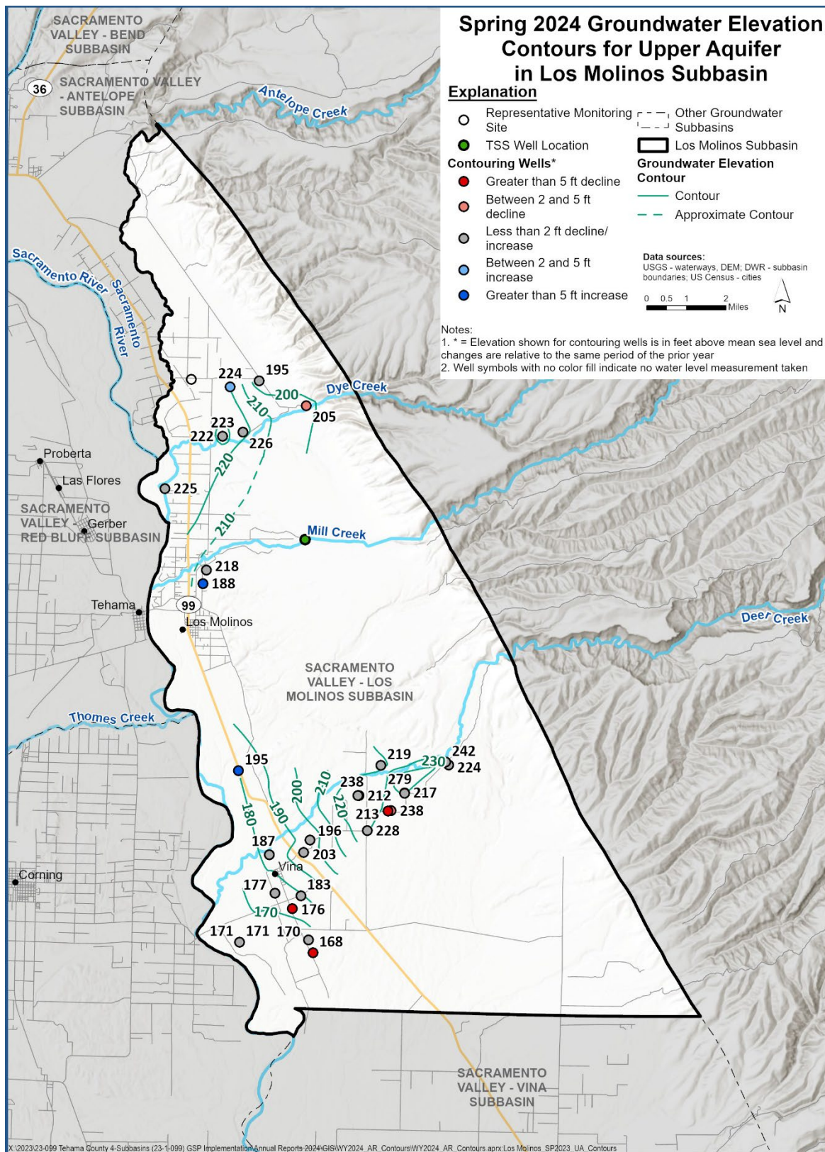
Figure 2-1. Los Molinos Subbasin Contours of Equal Groundwater Elevation for the Upper Aquifer, Spring 2024 (Seasonal High)
