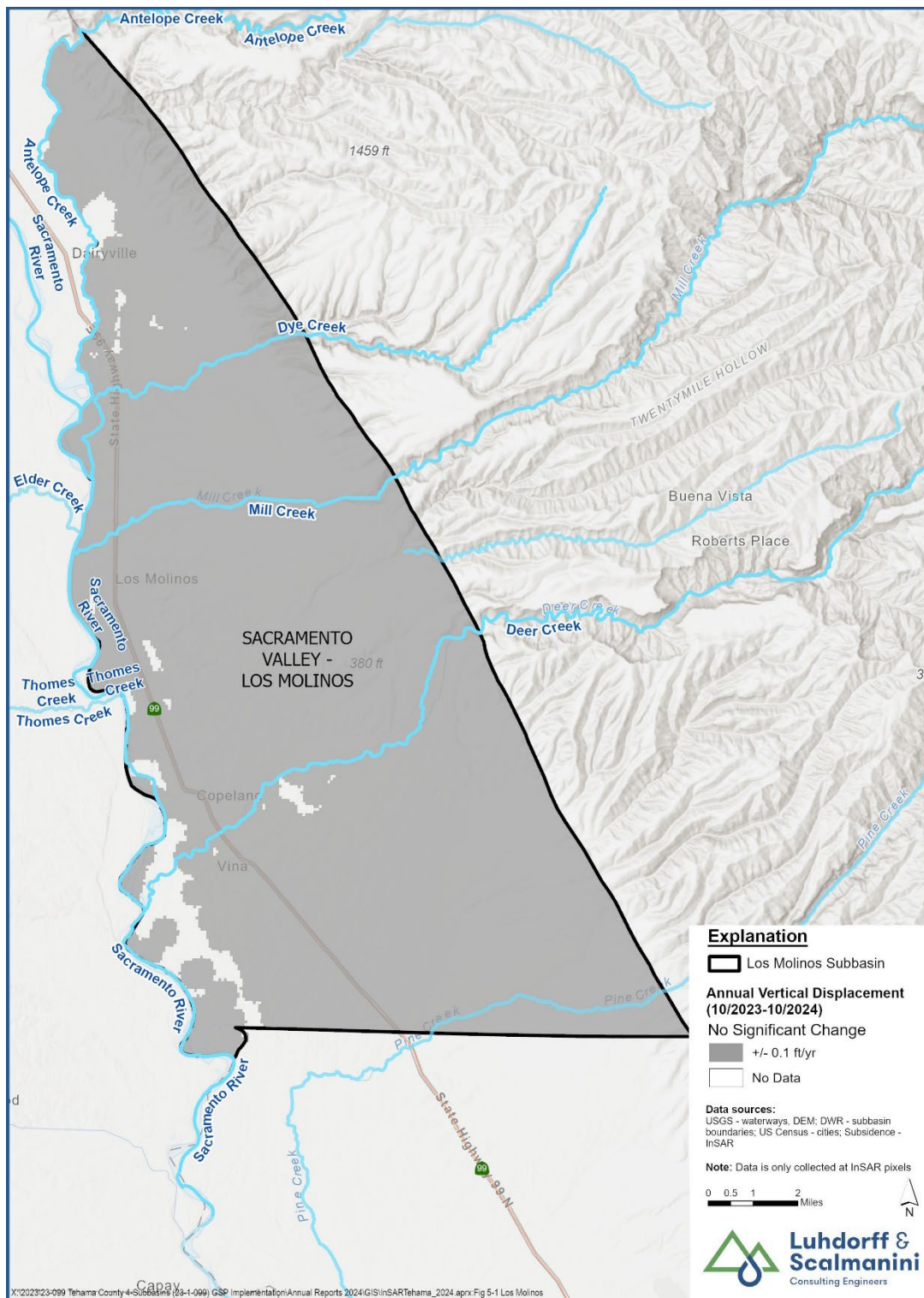
Figure 5-1. Los Molinos Subbasin Change in Subsidence from 10/2023 to 10/2024
