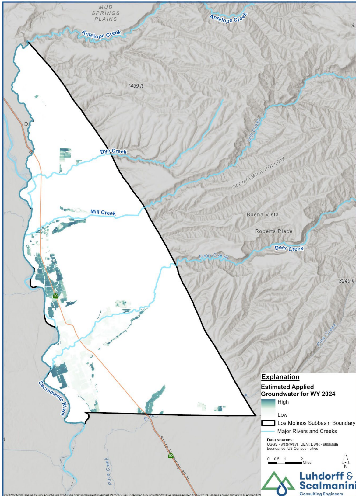
Figure 3-1. Los Molinos Subbasin Estimated Applied Groundwater – WY 2024
