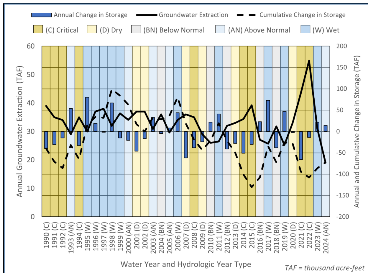
Figure ES-2. Los Molinos Subbasin Groundwater Pumping, Annual and Cumulative Change in Storage from WY 1990 to WY 2024
