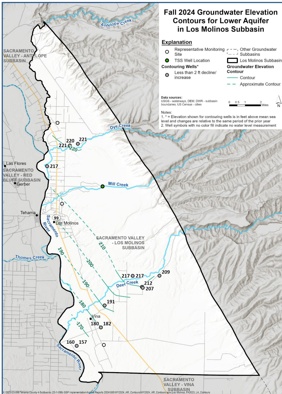
Figure 2-4. Los Molinos Subbasin Contours of Equal Groundwater Elevation for the Lower Aquifer, Fall 2024 (Seasonal Low)
