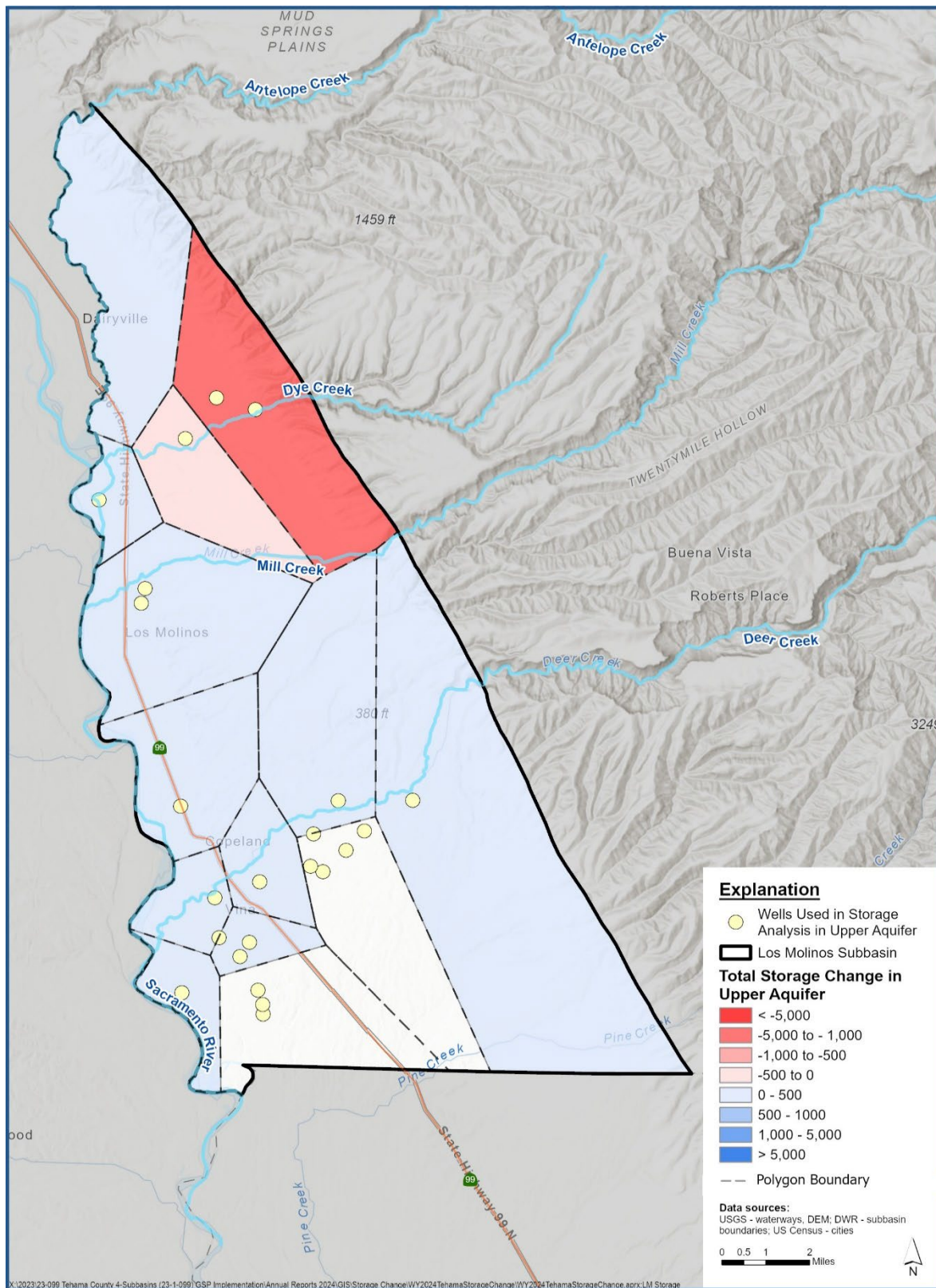
Figure 4-2. Los Molinos Subbasin Change in Groundwater Storage from Spring 2023 to Spring 2024 in the Upper Aquifer
