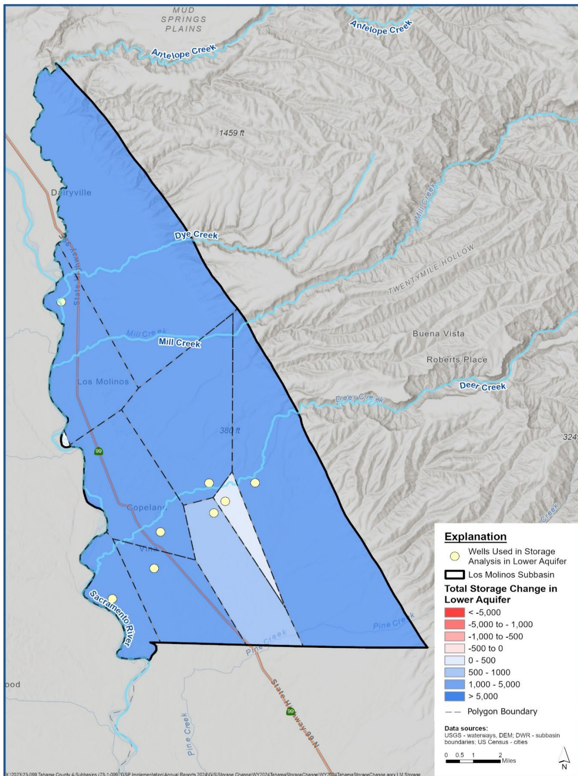
Figure 4-3. Los Molinos Subbasin Change in Groundwater Storage from Spring 2023 to Spring 2024 in the Lower Aquifer
