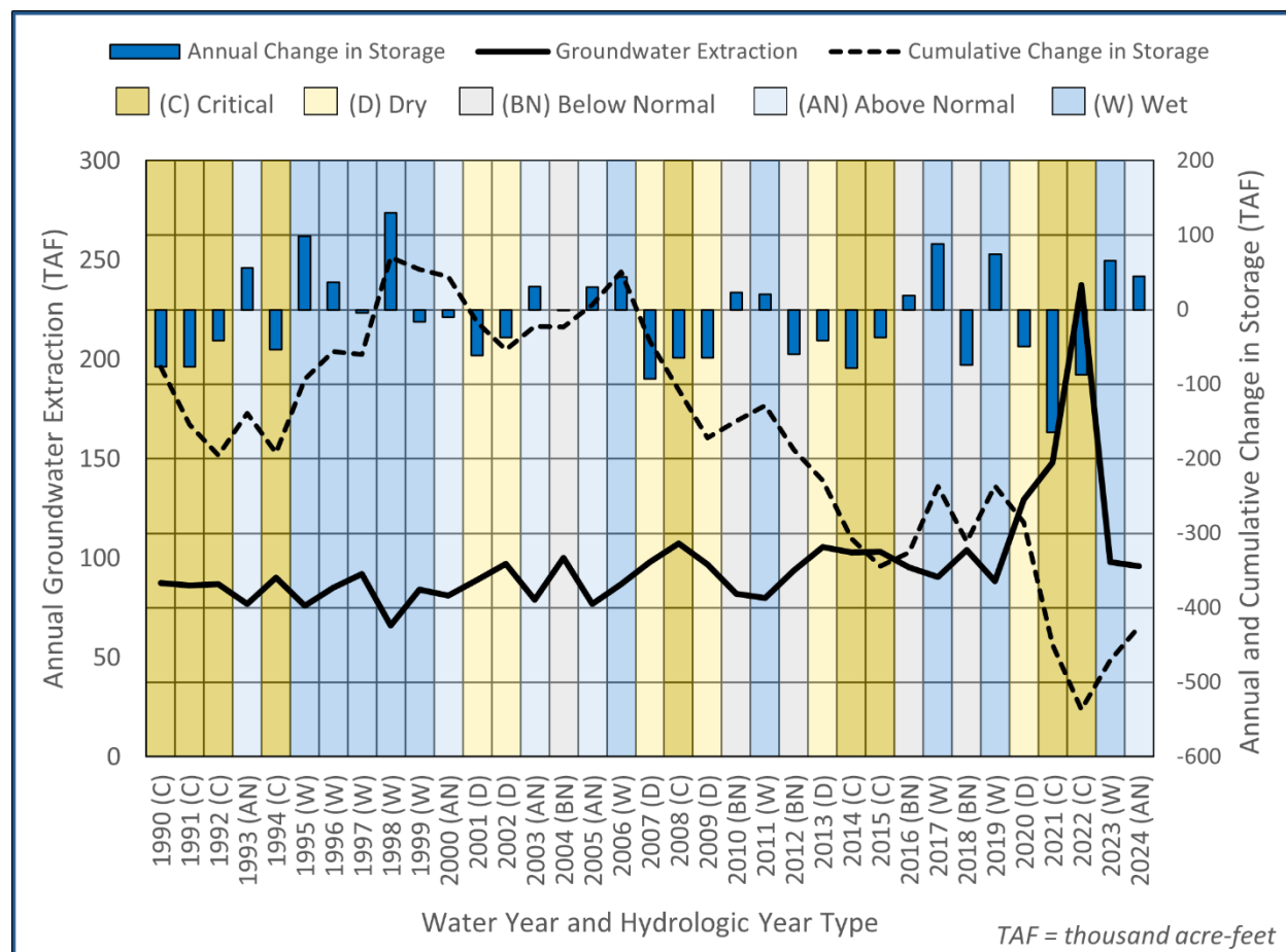
Figure 4-1. Red Bluff Subbasin Groundwater Extraction and Change in Groundwater Storage from WY 1990 to WY 2024
